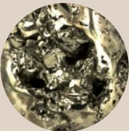
Golden Pyrite
