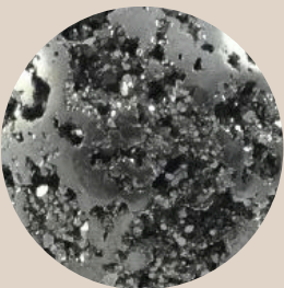
Silver Pyrite
