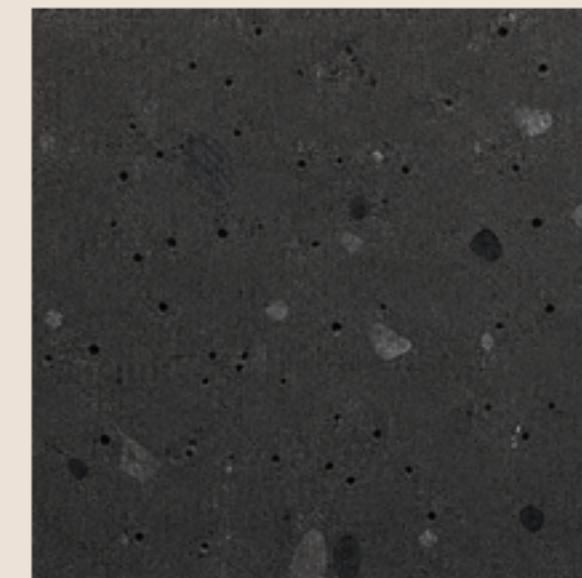
BASALT
