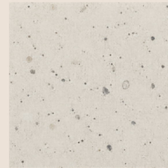
LIMESTONE
